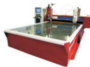
JETMax HS 12030, working area 12 x 3 m
